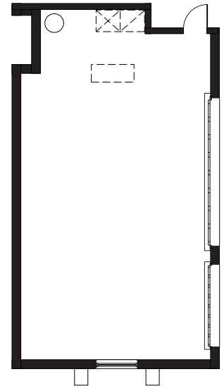
EXPANDED GARAGE - 5 FT WIDTH
