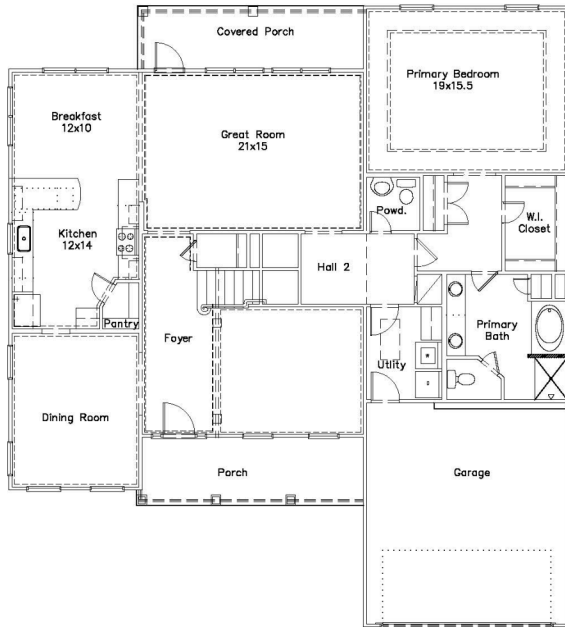
FIRST FLOOR PLAN (53'-4.5" x 59'-0")
