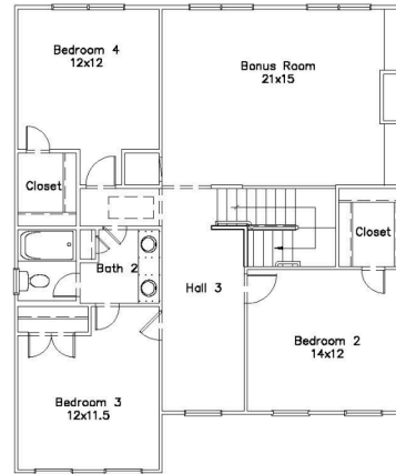
SECOND FLOOR PLAN (34'-0" x 40'-0")
