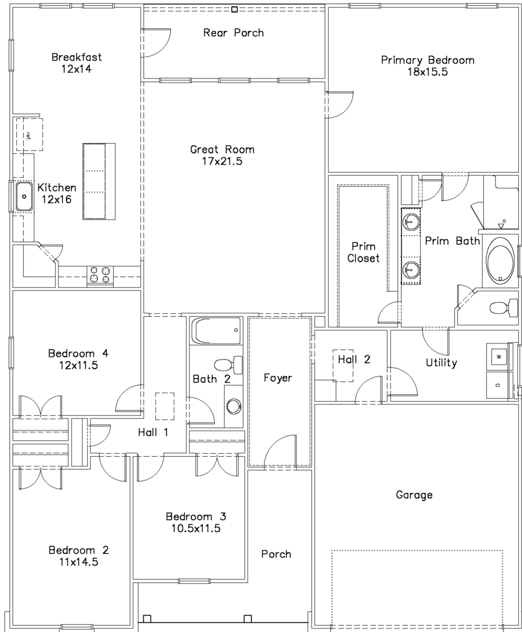
FIRST FLOOR PLAN (48'-11" x 59'-0")
