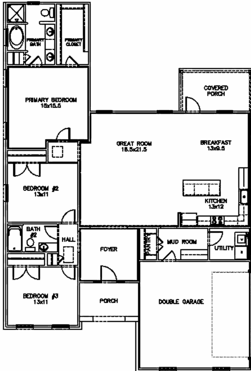
FIRST FLOOR PLAN W/ SIDELOAD GARAGE OPTION (47' x 68'-10")
