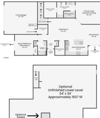
The Creekside Ranch Villa | 2BR | 2BA | 1507 SF | Optional Lower Level
