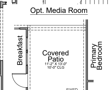
Opt. Sliding Patio Door @ Covered Patio
