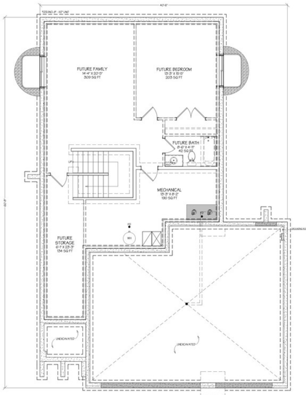
Cascade 3.0 - Base Plan - Lower Floor - 1,204 sq ft
