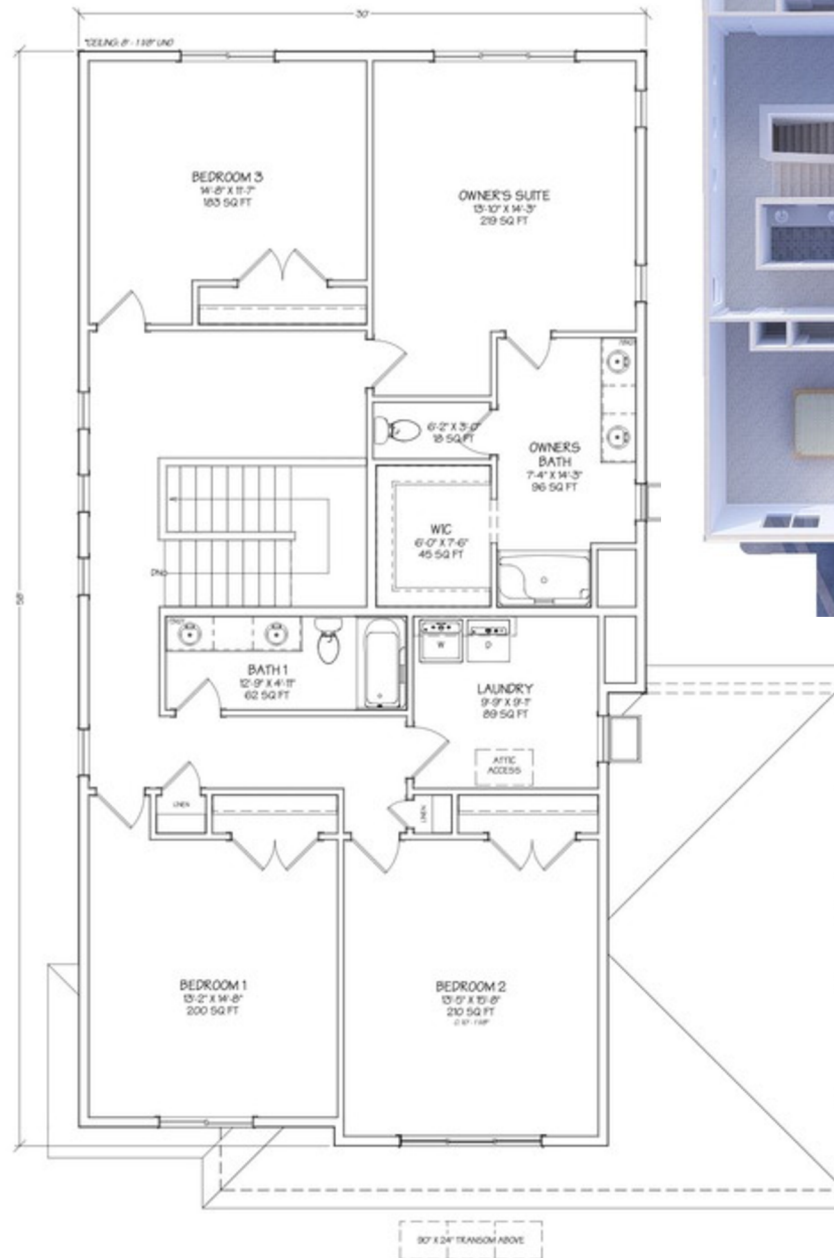
Cascade 3.0 - Base Plan - Upper Floor - 1,679 sq ft
