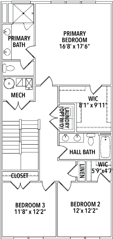
UPPER LEVEL WITH OPTIONAL TERRACE
