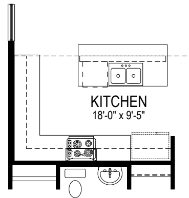
OPTIONAL DELUXE KITCHEN
