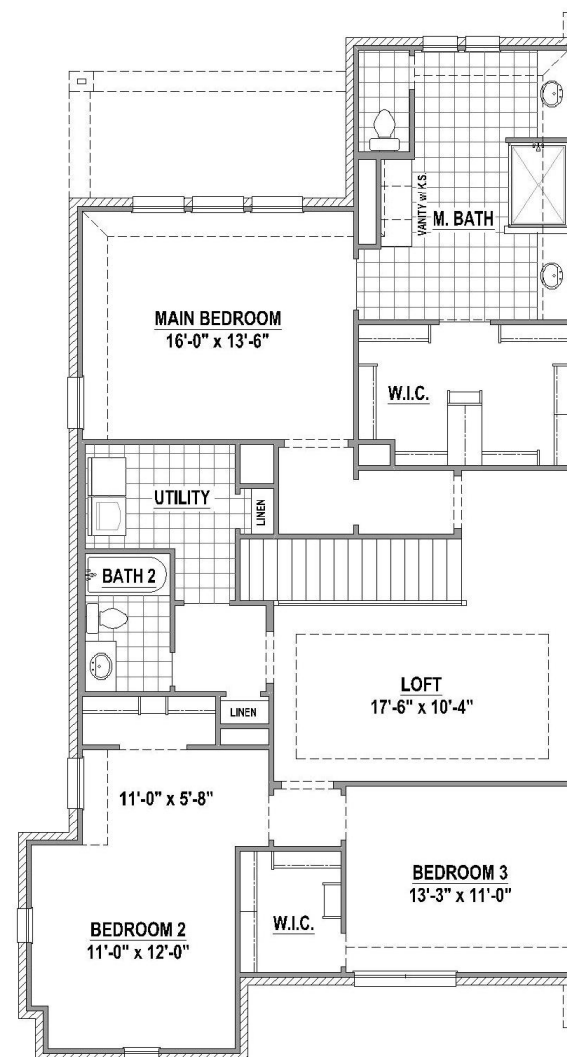
2 nd Floor
