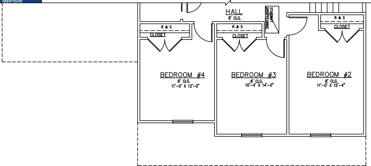
SECOND FLOOR PLAN OPT. E
