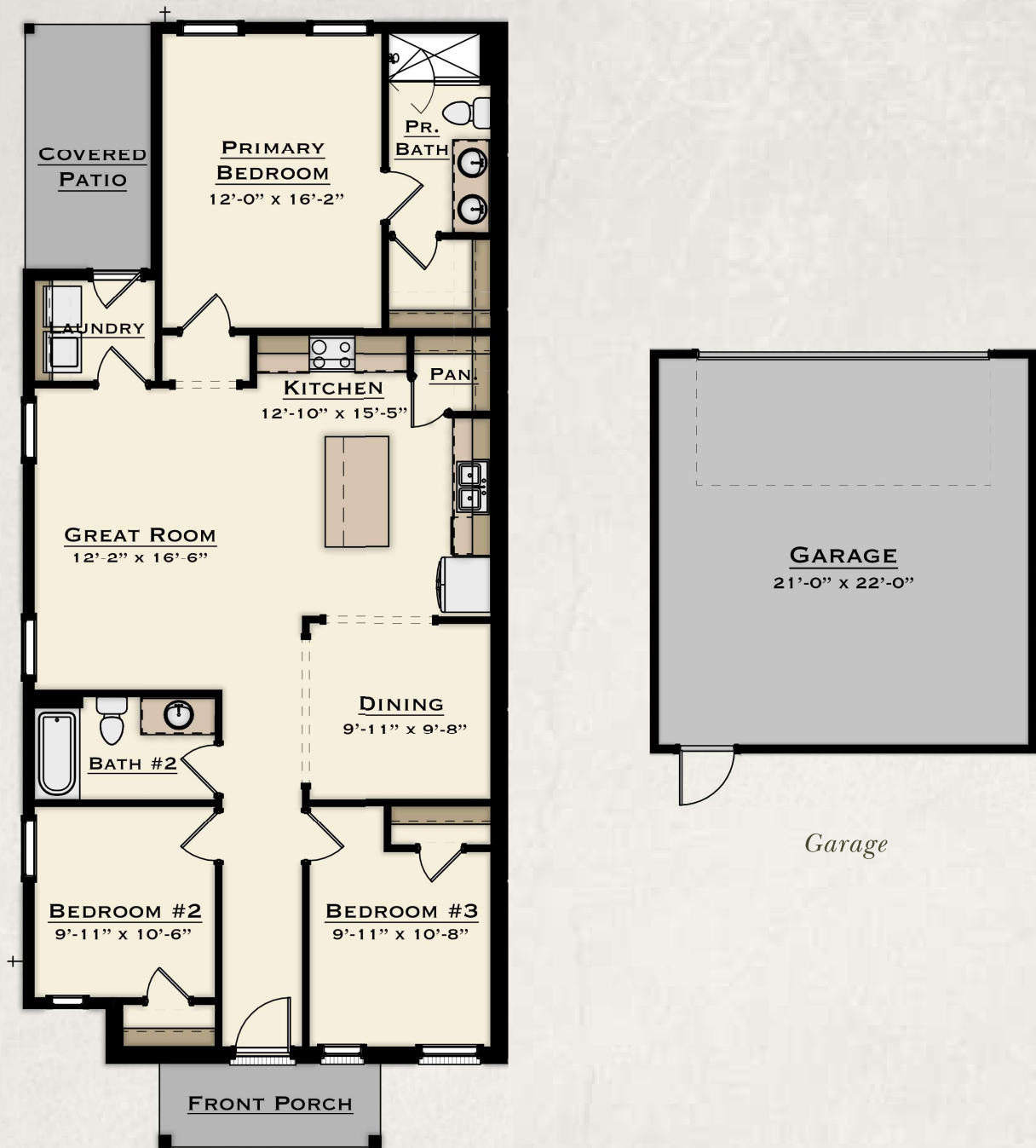
Main Level
