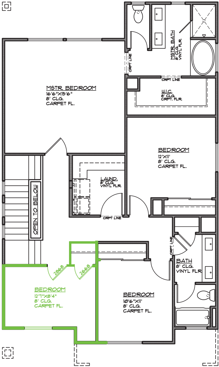
UPPER FLOOR PLAN UPPER FLOOR - 1213 SQ. FT.
