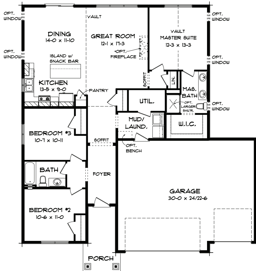
MAIN LEVEL
