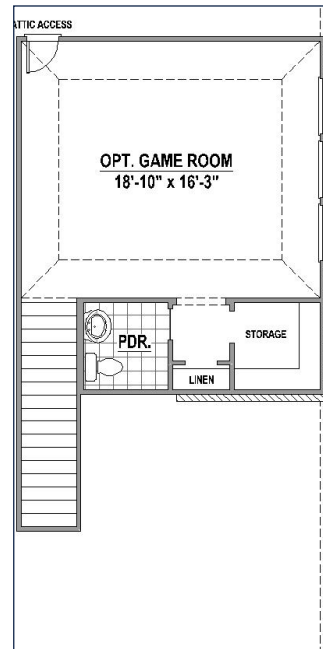
Game Room w/ Powder Bath (+433 SF)
