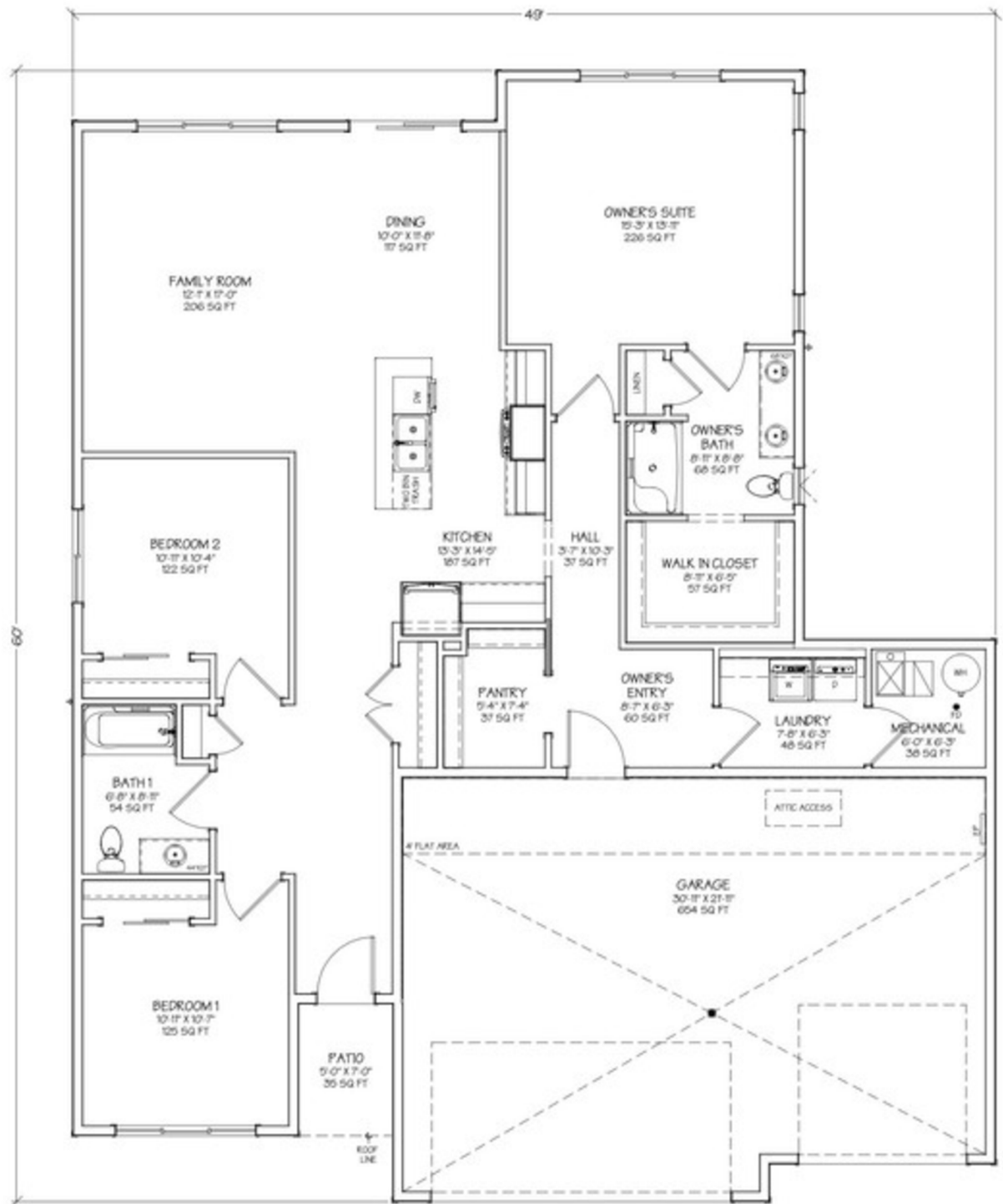
Dutton 3.0 - Base Plan - Main Floor - 1,765 sq ft
