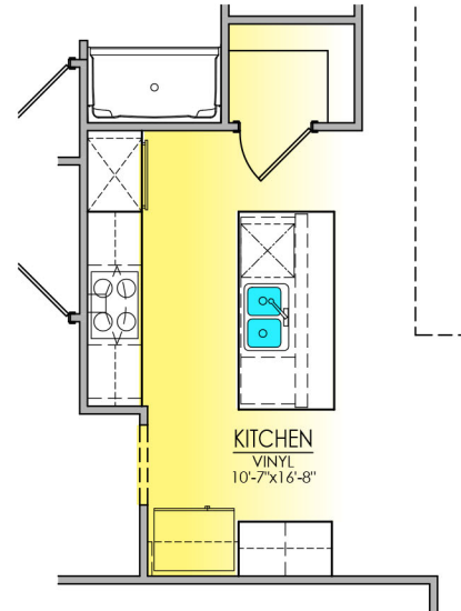
10 - OPT DELUXE KITCHEN
