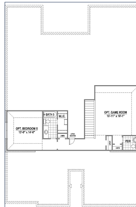
Optional Game Room and Bedroom 5 w/ Bath (+811 SF)
