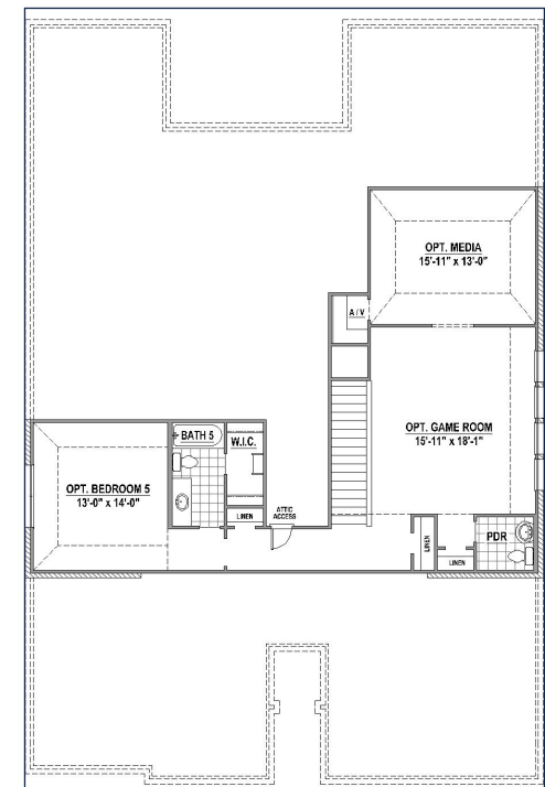
Game Room, Media Room and Bedroom 5 w/ Bath (+1,056 SF)
