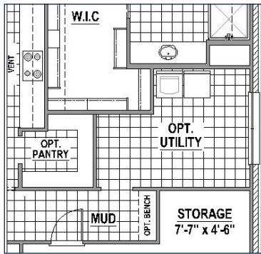
Walk-in Pantry & Utility Room (+122 SF)
