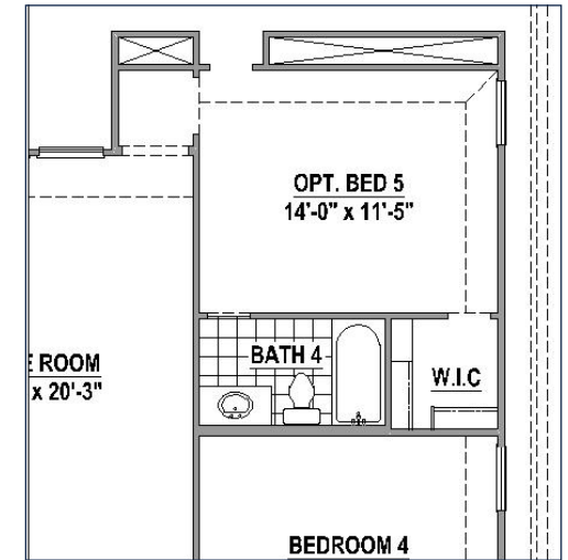
Bedroom 5 w/ Bath 4 (+261 SF)
