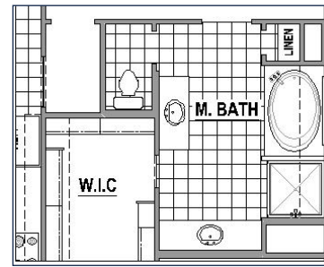
Drop-in Tub at Main Bath
