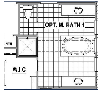
Alternate Main Bath Layout 1 (+93 SF) *not available with Walk-in Pantry & Utility
