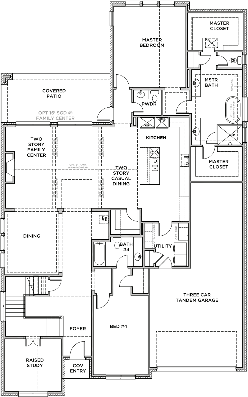
FIRST FLOOR
