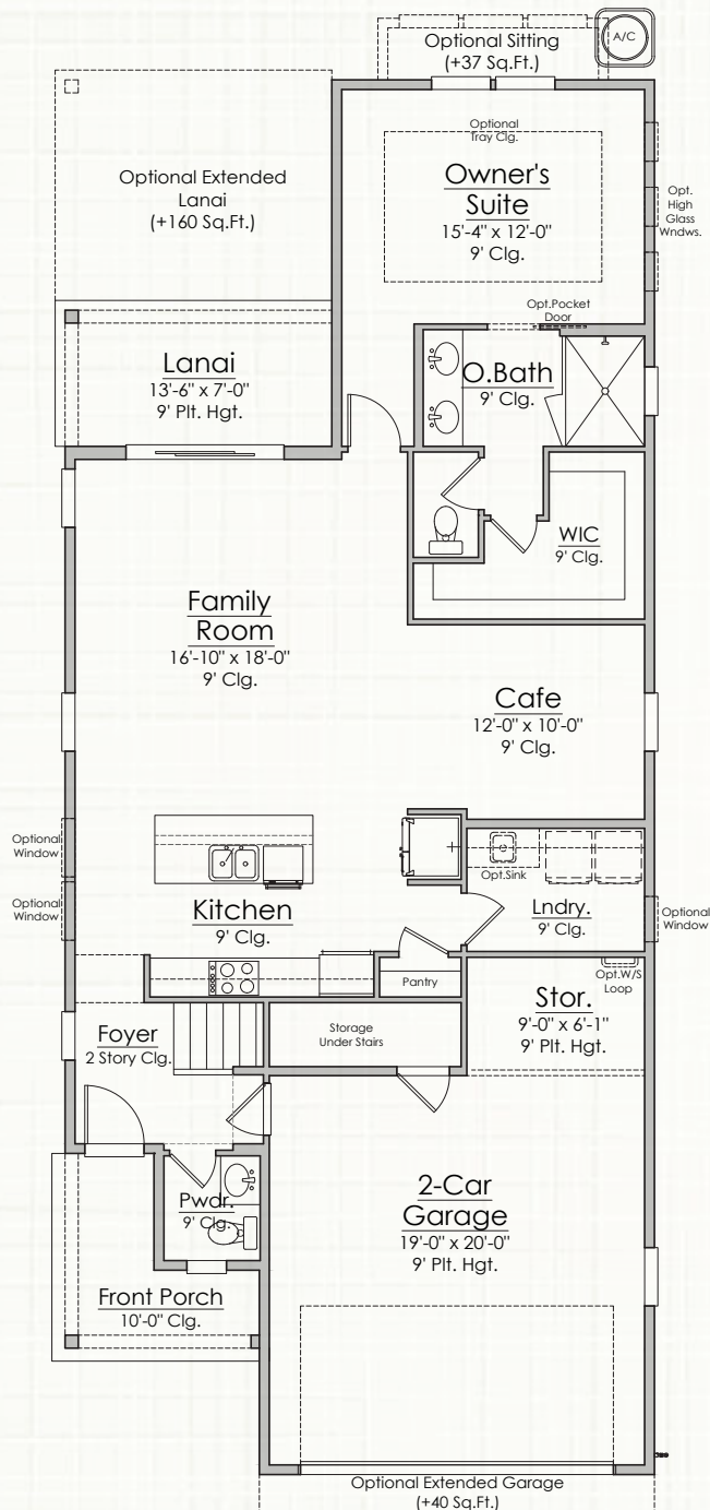
FIRST FLOOR
