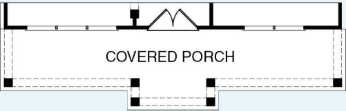
A1, A3 PARTIAL FLOOR PLAN
