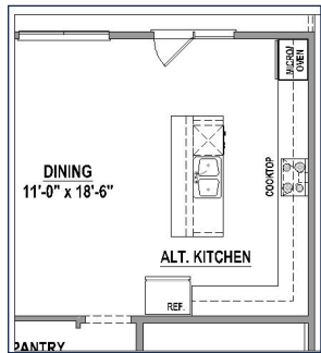
Alternate Kitchen Layout
