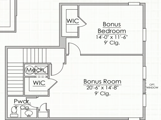
2nd Floor Plan with Bonus Bedroom (191 Sq.Ft.)
