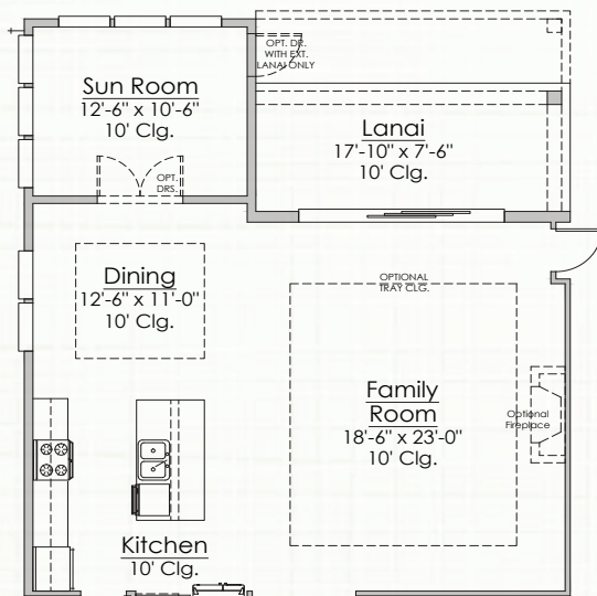
Optional Sun Room (162 Sq.Ft.)
