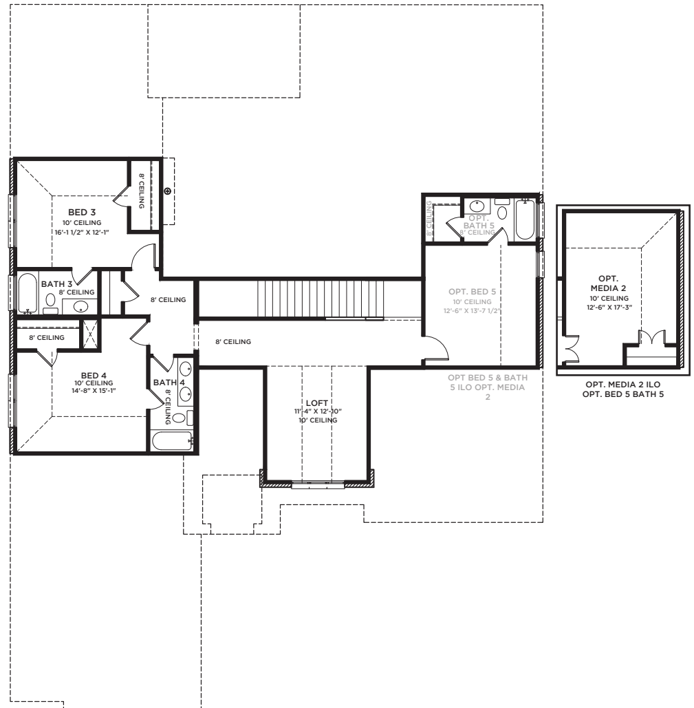
SECOND FLOOR
