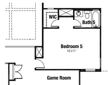
Bedroom 5/Bath 5 at 2nd Floor Option
