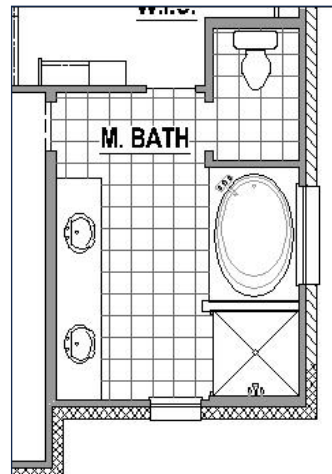
Alternate Main Bath Layout w/ Drop In Tub
