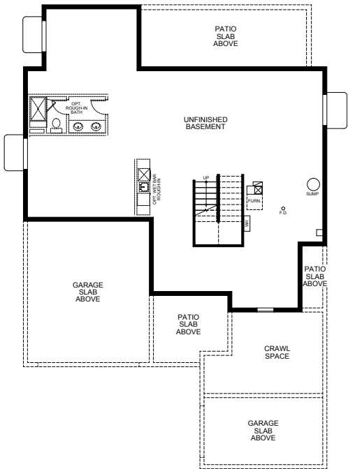
STANDARD UNFINISHED BASEMENT
