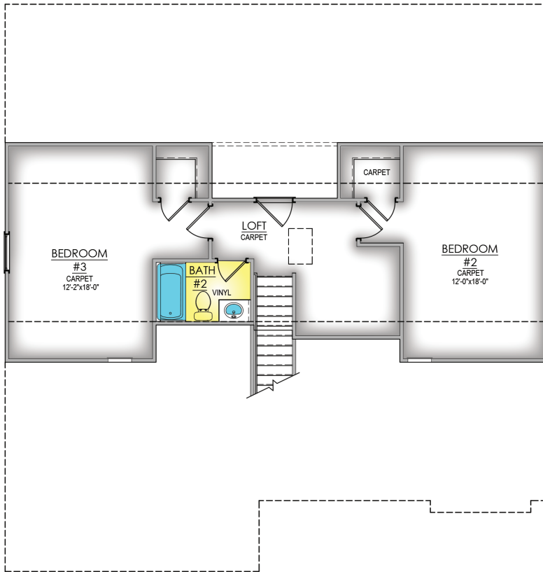
SECOND LEVEL - ELEV. A & B
