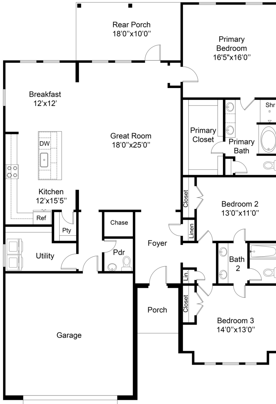
FLOOR PLAN
