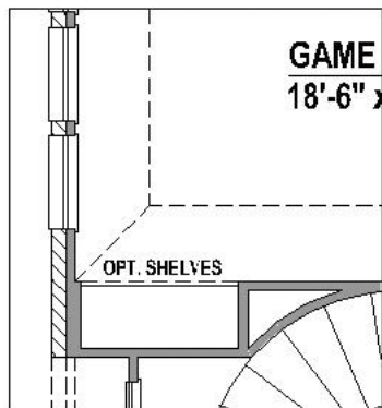
Optional Built-In Shelves in Game Room
