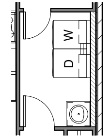
24" CABINET & 18" SINK IN UTILITY
