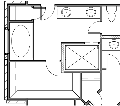
ALTERNATE MASTER BATH LAYOUT WITH EXTENDED CLOSET
