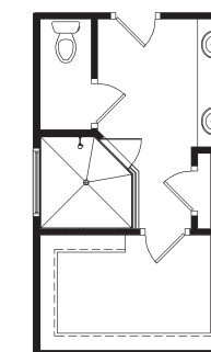
OPTIONAL OWNER'S BATH 3
