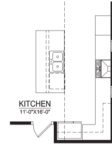
OPTIONAL PRESTIGE KITCHEN
