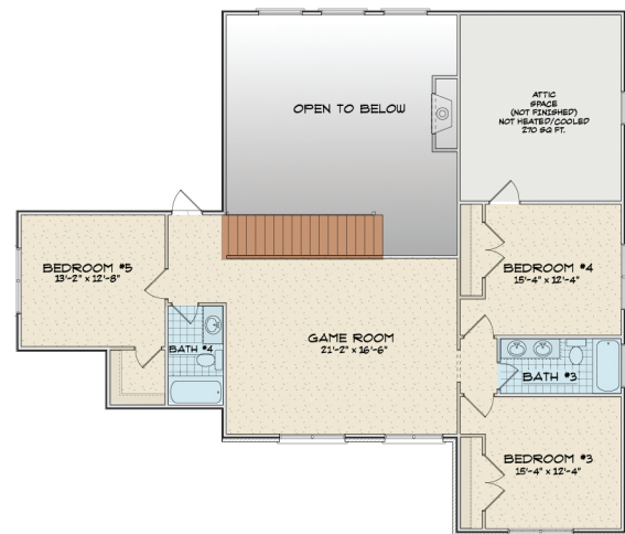
Upper Level Floor 1,159 sf
