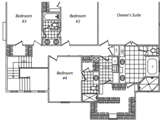
2nd Floor Plan 1605 sq ft
