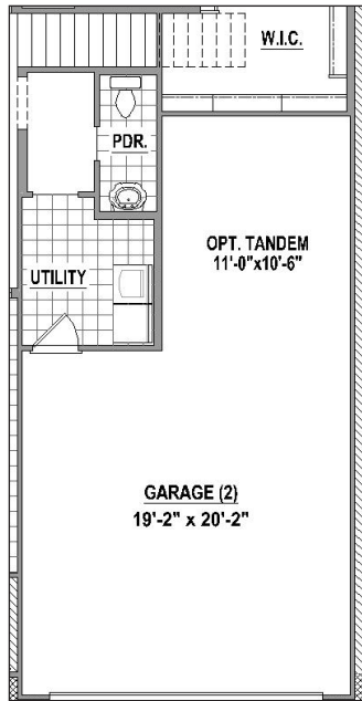
Tandem Garage w/ Stairs to 2nd Floor Options (-161 SF)
