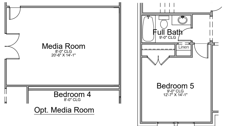
Opt. Bedroom 5 w/ Full Bath into Flex Room
