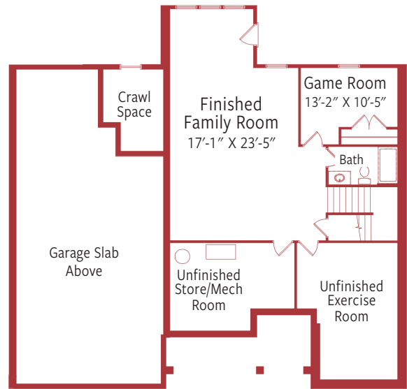
Optional Finished Basement, Optional Finished Bath, Optional Finished Game Room & Optional Closet
