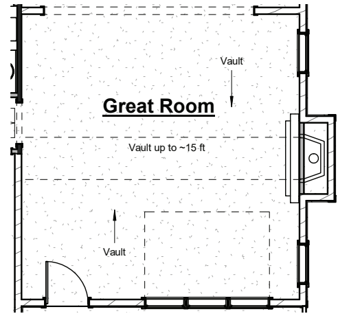
Great Room Fireplace Bump-Out
