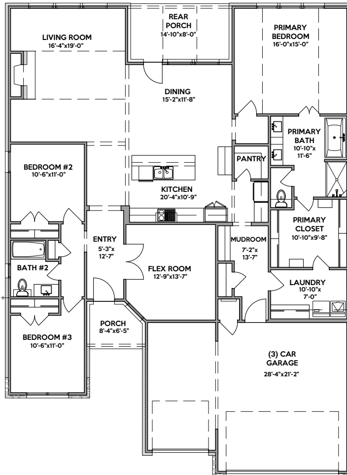
FIRST FLOOR ELEVATION "A", "C" & "D"
