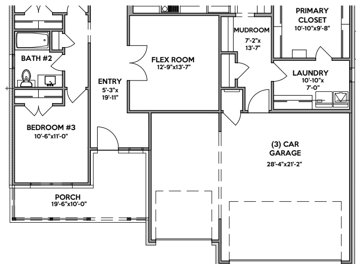
FIRST FLOOR ELEVATION "B" (APPROX. 63 SQ FT MORE)
