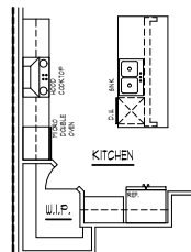
OPTIONAL BUILT-IN DOUBLE OVEN KITCHEN APPLIANCES
