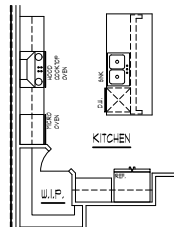
OPTIONAL BUILT-IN W/ OVEN AT COOKTOP KITCHEN APPLIANCES
