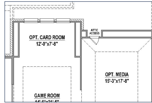
Card Room and Media Room (+396 SF)
