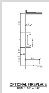
OPTIONAL FIREPLACE (W/ BUILT-INS)
