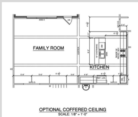
OPTIONAL COFFERED CEILING
