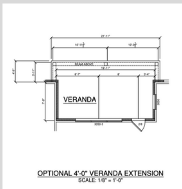
OPTIONAL 4' VERANDA EXTENSION
