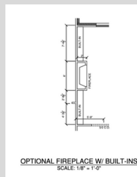
OPTIONAL FIREPLACE (W/ BUILT-INS)
