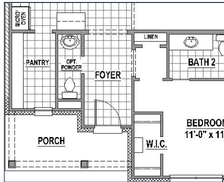
Powder Bath ILO Linen Closet at Entry
