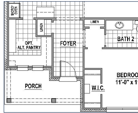
Alternate Pantry Layout
