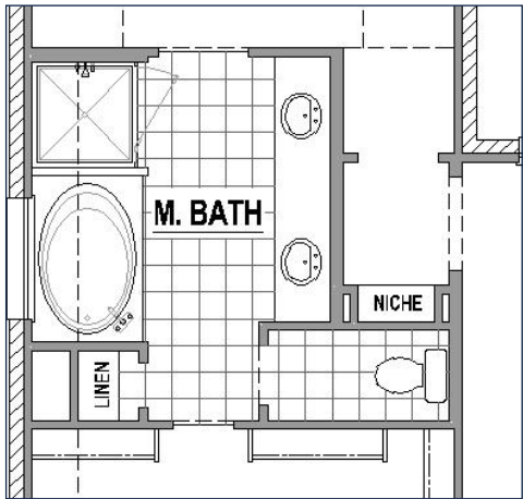
Optional Drop in Tub at Main Bath
