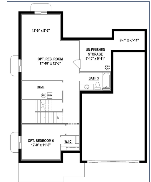
Rec Room w/ Bedroom 6 & Bath 3 (+843 SF)
