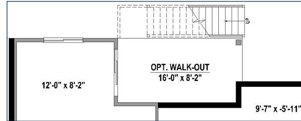
Walk-Out Basement
