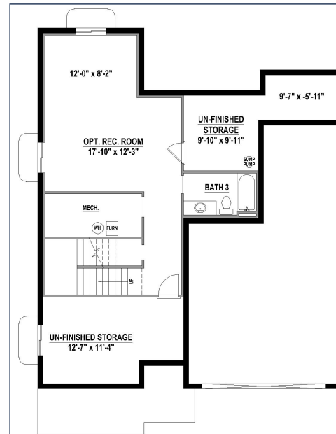
Rec Room w/ Bath 3 (+632 SF)
