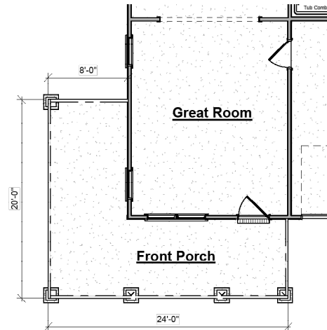
Wrap Around Front Porch
