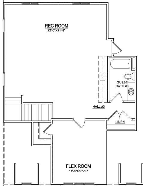
Optional 2 nd Floor #1 add 920 sq. ft.
