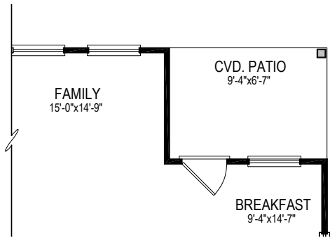
OPTIONAL COVERED PATIO
