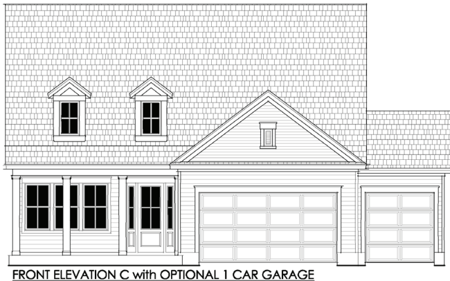
ELEVATION C
